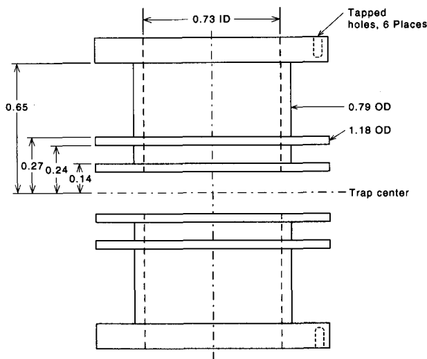
Fig. 6. Mechanical drawing of coil assembly. Dimensions in inches, with only critical dimensions shown. Wire coils are wound within the channels. Tapped screw holes are located equilaterally about the top and the bottom coil form.
