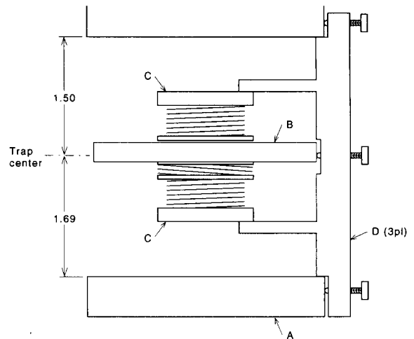
Fig. 5. Drawing of the apparatus. Dimensions are in inches. Parts A are toroidal iron magnets, with outer diameter 2.9, inner diameter 1.2, and thickness 0.5. Part B is a trim magnet with OD 2.6, ID 2.1, and thickness 0.25. The position of part B relative to trap center is adjustable by set screws. Parts C are the coil assembly, shown in detail in Fig. 6. Parts D are three aluminum support posts, bolted to parts C.
