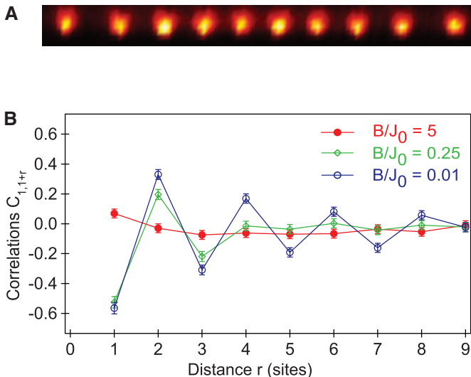
Fig. 3. Quantum phase transition from a paramagnet to an antiferromagnet (Eq. 1), with J_{ij} \approx |i - j|^{-1.05} in a system of 10 spins. The exponent ( \alpha = 1.05 ) is estimated from the average couplings between spins in this inhomogeneous system. (A) Image of 10 trapped ions, with a distance of 22 \mu\text{m} between the first and last ion. (B) Measured two-point correlation function between a chosen spin (on the edge) and the other spins separated by r lattice sites, C_{1,1+r} = \langle \sigma_x^{(1)} \sigma_x^{(1+r)} \rangle - \langle \sigma_x^{(1)} \rangle \langle \sigma_x^{(1+r)} \rangle , averaged over 4000 experiments for each value of the parameter B/J_0 . For B/J_0 = 5 , the spins are initially polarized along the transverse y field with little correlation along the Ising x direction. As the field is reduced, the spins cross over to pre-
