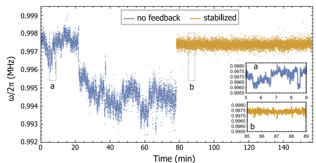
FIG. 7. Time dependence of the ion harmonic oscillation frequency \omega plotted over the course of 160 min with and without active stabilization. With feedback there is a clear reduction in noise and drifts (apart from measurement shot noise, reflected by the fast fluctuations in the data). Inlays a and b show magnified sections of the plot covering 4 min of integration.
