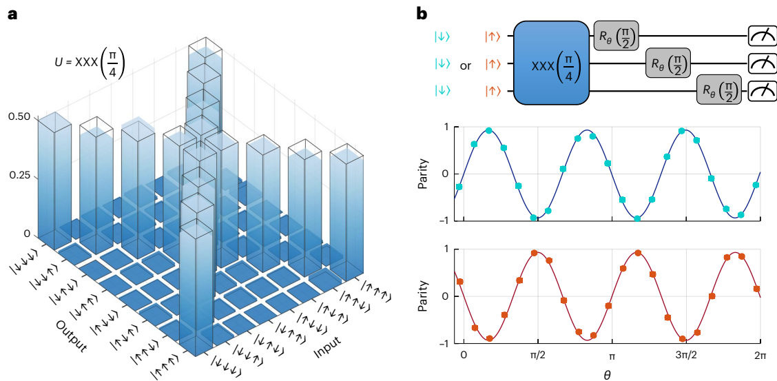
Fig. 3 | Characterization of a three-body interaction gate. a , Truth table of a three-body gate XXX(\frac{\pi}{4}) = \exp(-i\frac{\pi}{4}\sigma_x^{(1)}\sigma_x^{(2)}\sigma_x^{(3)}) generated by a sequence of displacement and squeezing operations. The input and output spin states are along the z basis. Each input state is ideally mapped into a pair of output states (wire frames), and the raw measurements are shown as the solid bars. The measured populations of these target states are (95.8 \pm 0.9)\% , averaged over the eight measured configurations. b , Characterization of the parity fringe witness observable obtained by the gate. We measure the parity fringe of the output GHZ state for the two initial states |\downarrow_z^{(1)}\downarrow_z^{(2)}\downarrow_z^{(3)}\rangle (light blue) and |\uparrow_z^{(1)}\uparrow_z^{(2)}\uparrow_z^{(3)}\rangle (red) with
