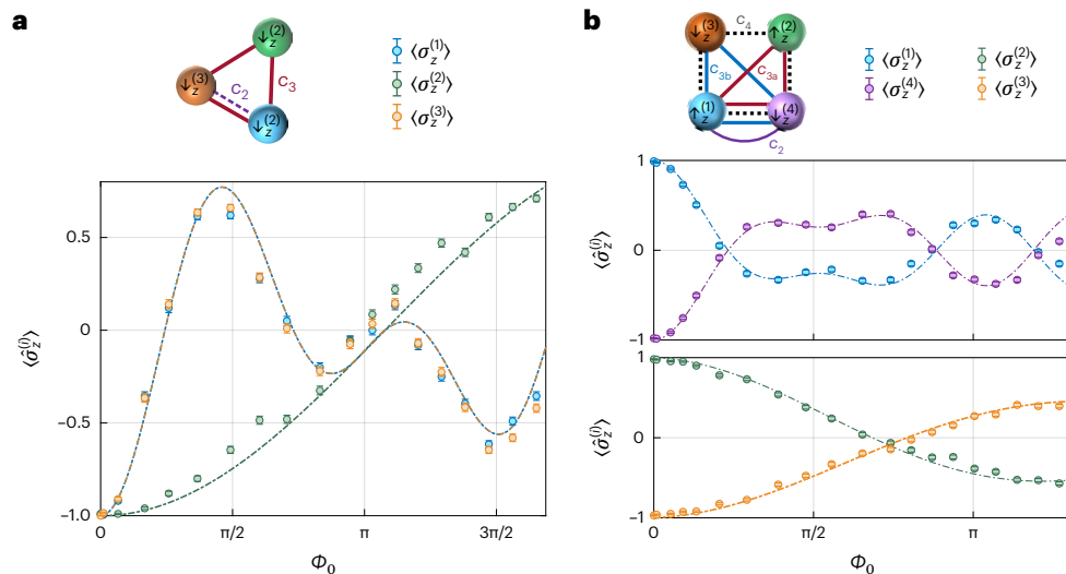
Fig. 4 | Evolution by effective Hamiltonians with three- and four-body interactions. a , Spin magnetization \langle \sigma_z^{(n)} \rangle under displacement and squeezing operations (Extended Data Fig. 1b) shown as a function of \Phi_0 for the initial state |\downarrow_z^{(1)}\downarrow_z^{(2)}\downarrow_z^{(3)}\rangle . Mathematically, this dynamics is equivalent to the evolution generated by the effective Hamiltonian H_{\text{eff}} = \Phi/\Phi_0 for \Phi in equation (1). The effective Hamiltonian comprises two- and three-body terms with magnitudes c_2 = 1.03 and c_3 = 0.23 , as illustrated via the links connecting the different spins. Here \Phi_0 has the role of the effective evolution time (in units of \hbar = 1 ) and is controlled by the amplitude of the Raman beams (described in the main text). b , Evolution of four spins by the displacement and squeezing operations
